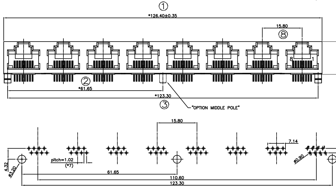
PC Board Layout Component Side Shown PC Board Thickness=1.6mm Tolerance±0.05
